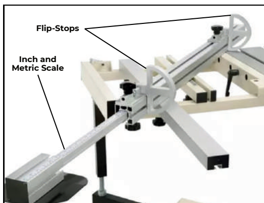
Crosscut fence for making repeat 90° and angled cuts up to 78" wide on large panels.
