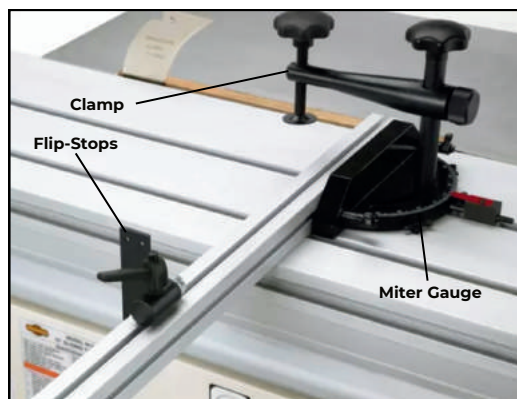
Miter fence with clamp and adjustable flip-stop for crosscutting and mitering smaller workpieces.
